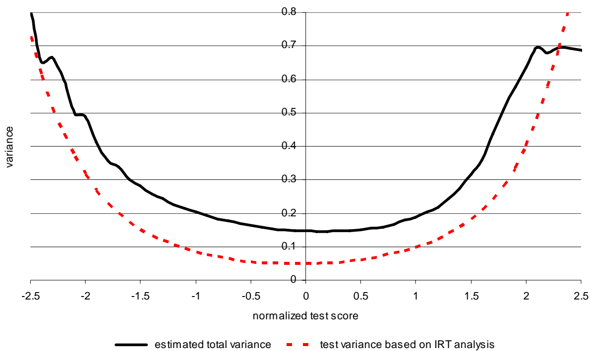
Figure 1 Estimated Total Measurement Error Variance and Average Variance of Measurement Error Associated with the Test Instruments (IRT Analysis) Grades 4-8 and Years 1999-2007
